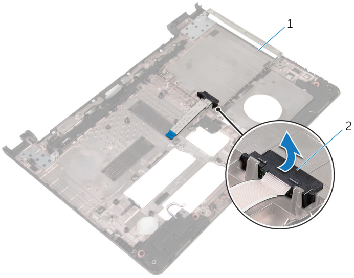
1 computer base
